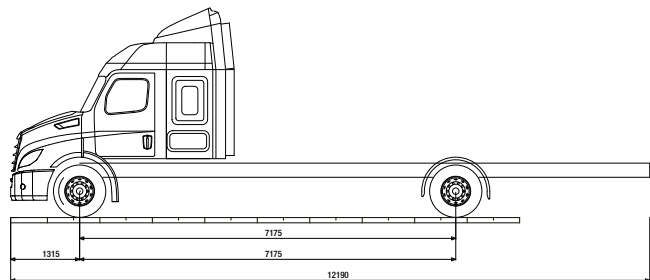
48" XT Sleeper Cab 4x2 4x2 only available in 48" XT Sleeper
