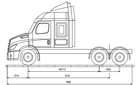
48" XT SLEEPER CAB
